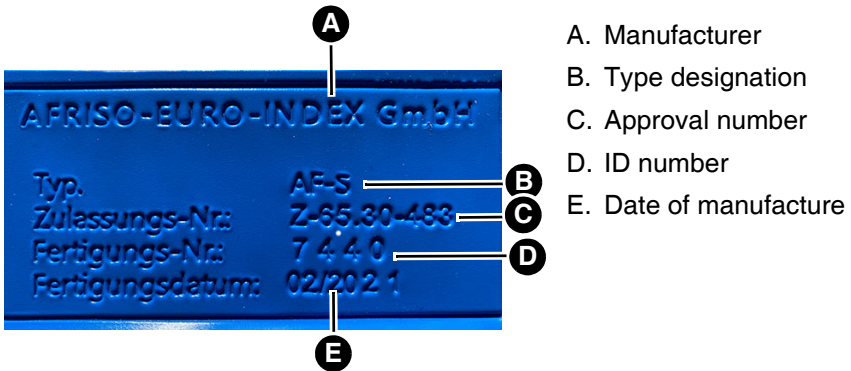
Fig. 1: Nameplate example
