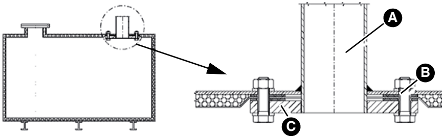
Fig. 2: Holes in tank ceilings
